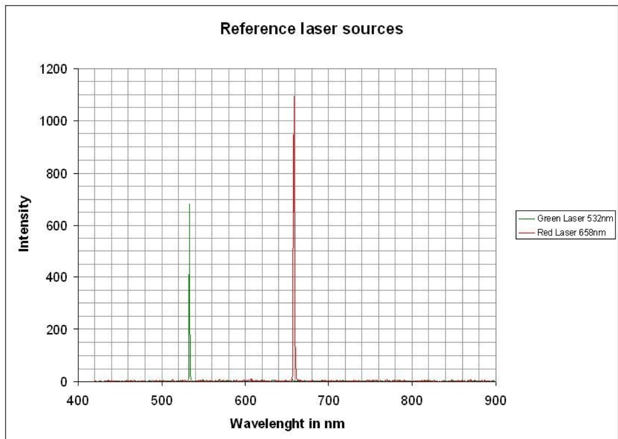
Figure1: Reference Lasers
