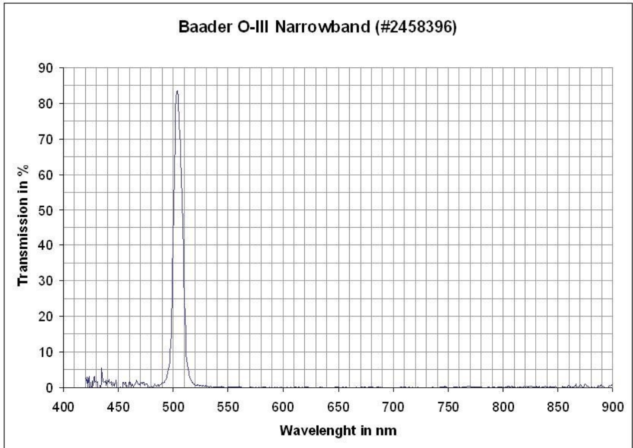
Figure 3: 2" Baader O-III
